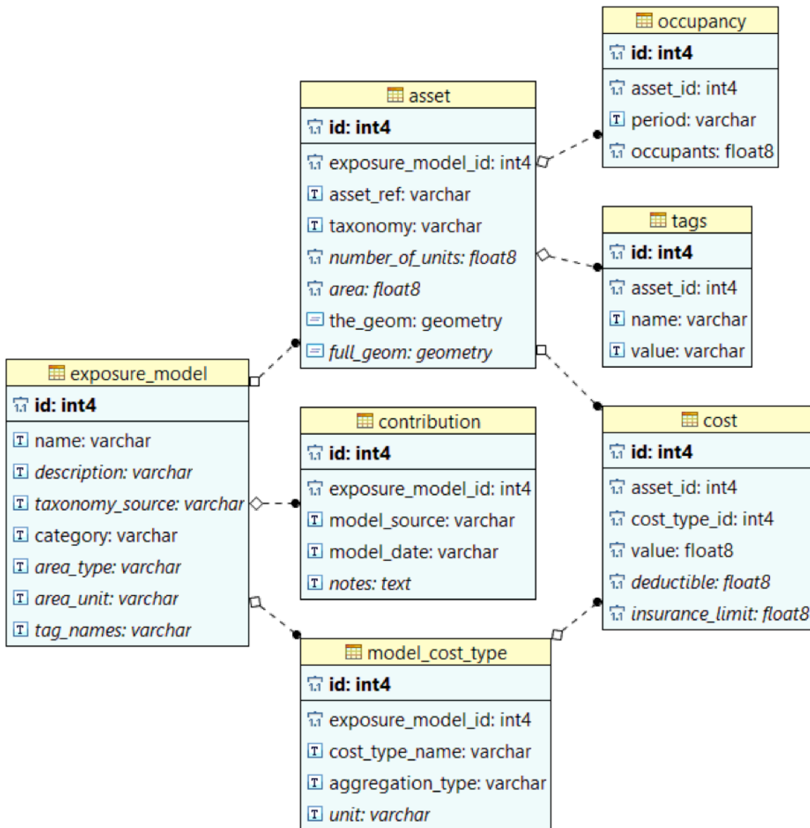
Figure 2 - GED4ALL Level 2 Schema Entity Relationship Diagram.
